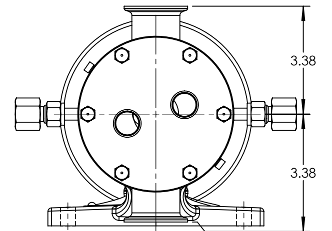
VERTICAL PORT ORIENTATION
