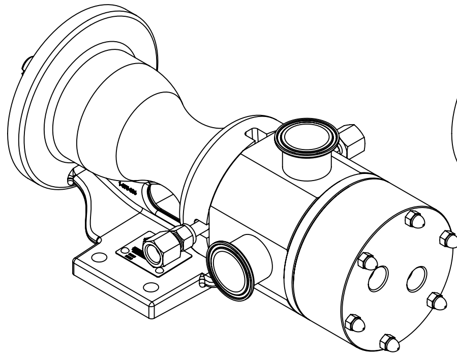
RIGHT HAND PORT ORIENTATION
