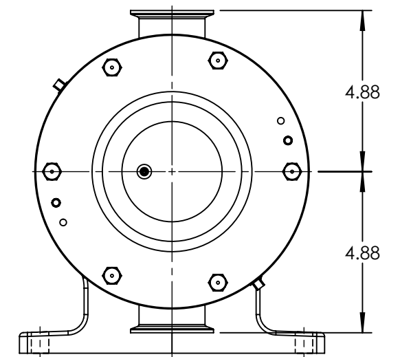
VERTICAL PORT ORIENTATION
