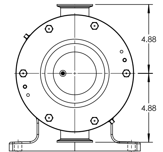
VERTICAL PORT ORIENTATION
