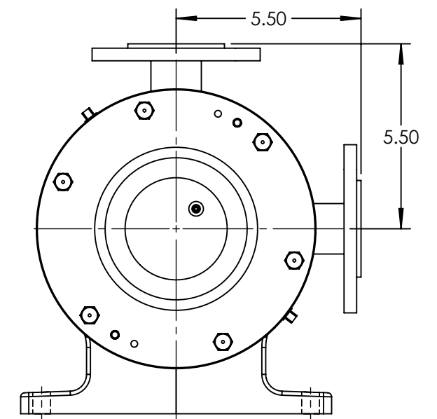
LEFT HAND PORT ORIENTATION
