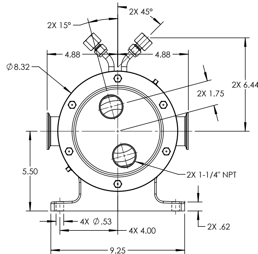
HORIZONTAL PORT ORIENTATION
