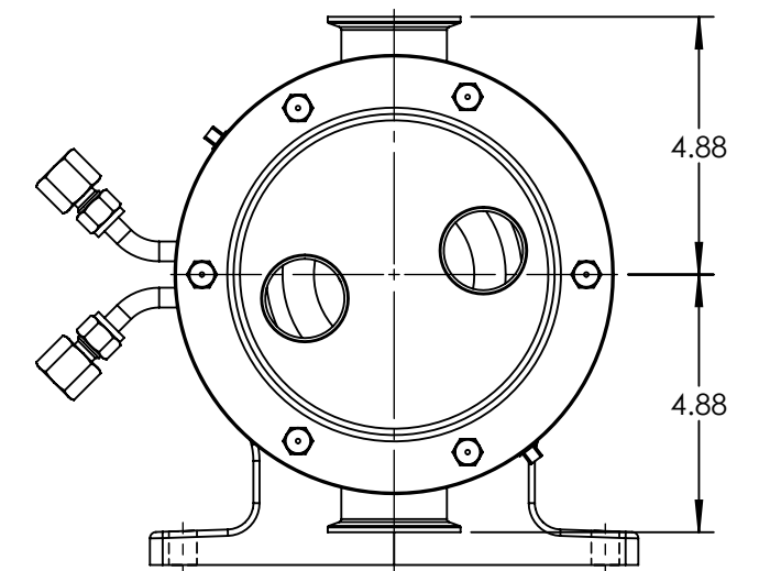
VERTICAL PORT ORIENTATION
