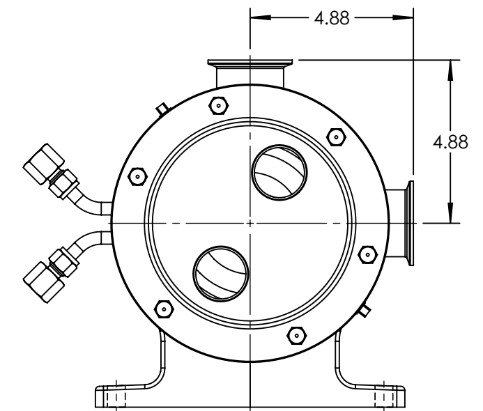
LEFT HAND PORT ORIENTATION
