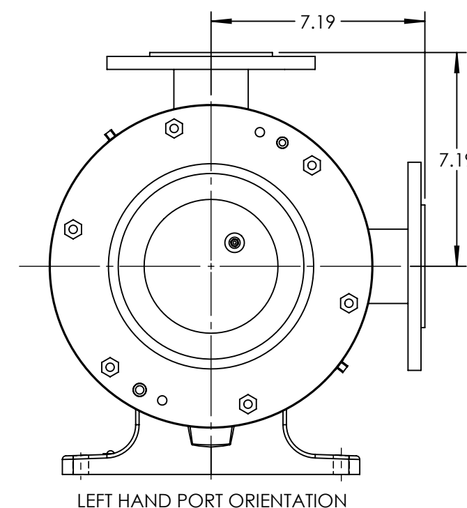
LEFT HAND PORT ORIENTATION
