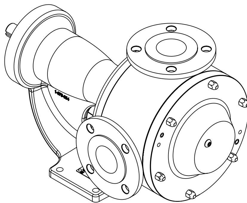
RIGHT HAND PORT ORIENTATION
