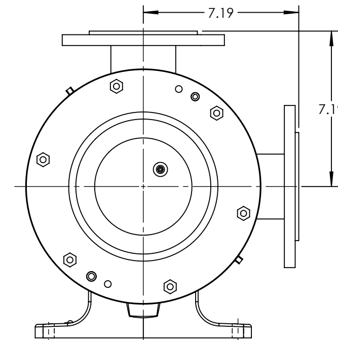
LEFT HAND PORT ORIENTATION
