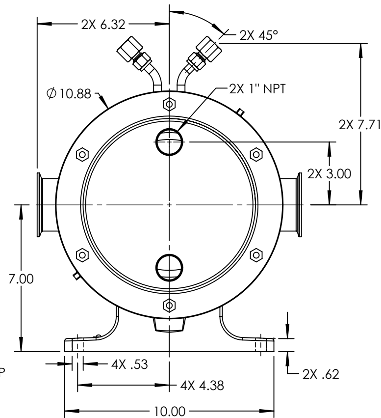
HORIZONTAL PORT ORIENTATION
