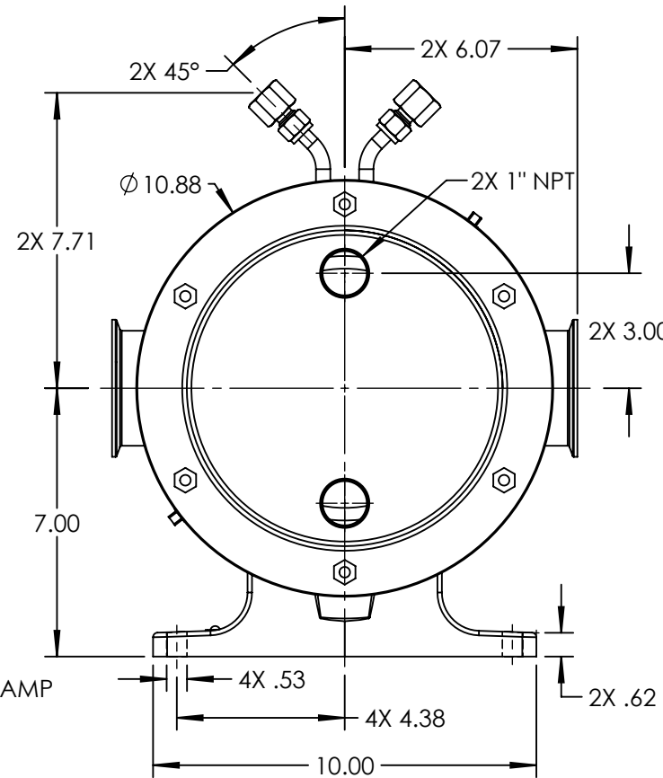
HORIZONTAL PORT ORIENTATION
