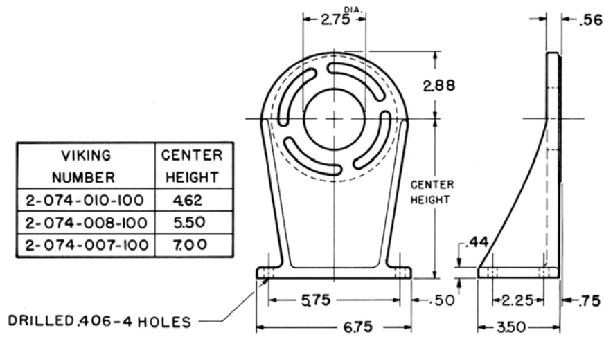
"B" SIZE BRACKET
