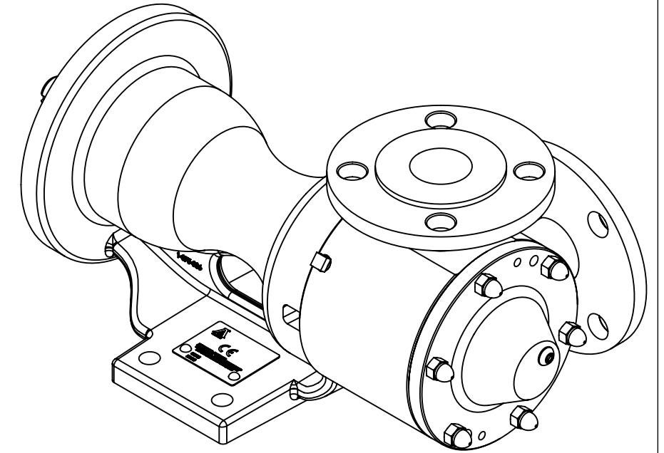
LEFT HAND PORT ORIENTATION
